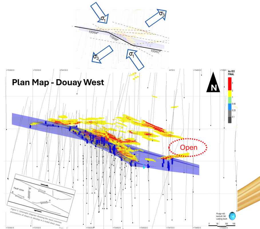
Figure 2: Plan map showing structural control on gold mineralization at the Douay West zone.
