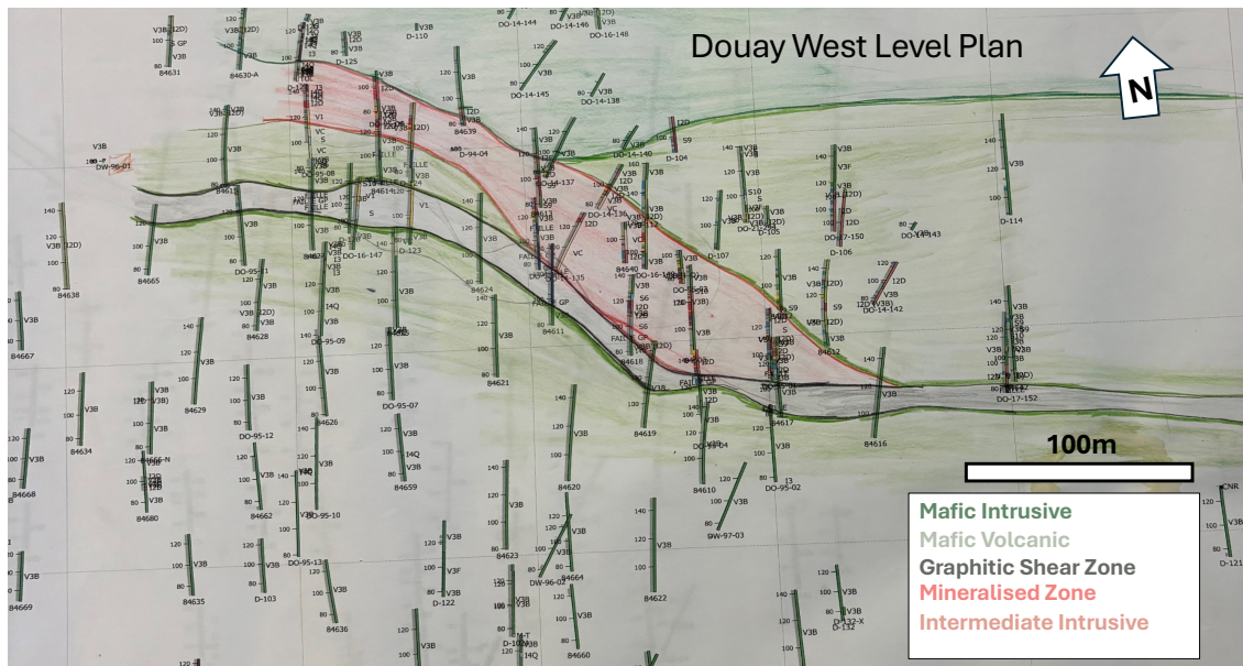
Figure 1: Hand-drawn Plan Level showing structural control on gold mineralization at the Douay West zone
