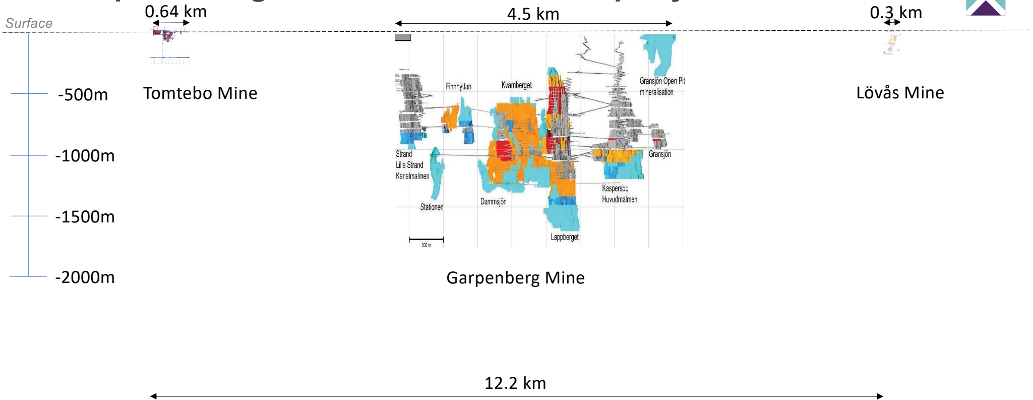
Conceptual Long Section Looking Northwest
