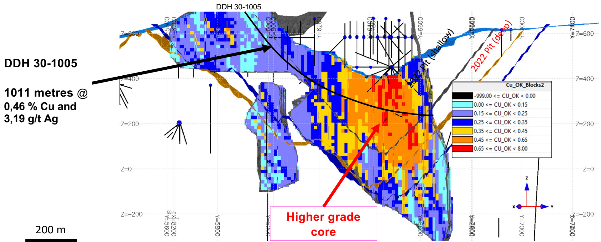
Block model in vertical section looking SW
