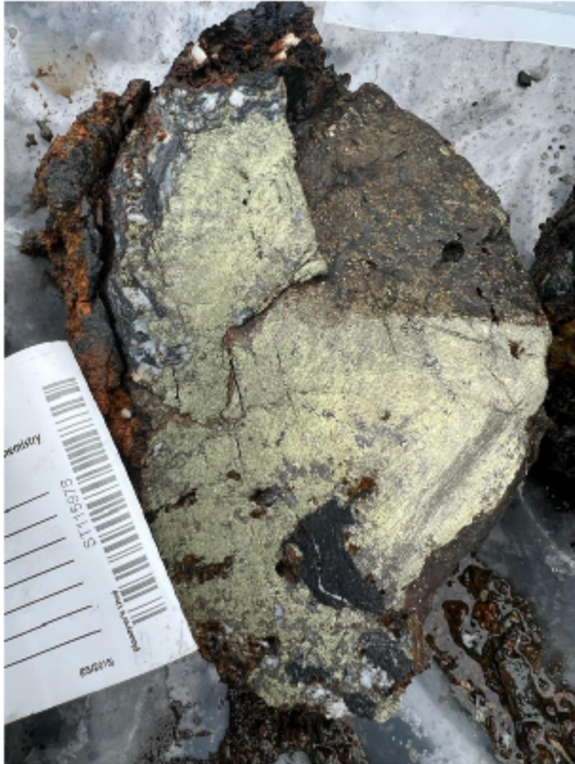
Samples from brecciated shears and veins with massive chalcopyrite and pyrite
