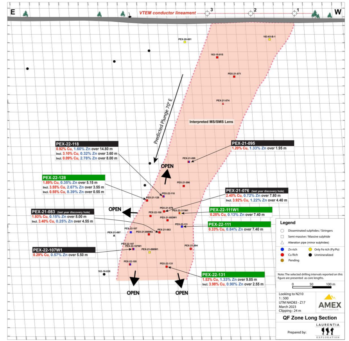
Note: The drill intervals for the QF zone are presented in core lengths.
