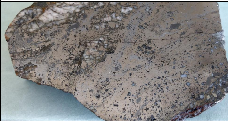
Representative channel sample from the Main Surebet zone Grading 7.66 g/t Au Eq over 8.4m
