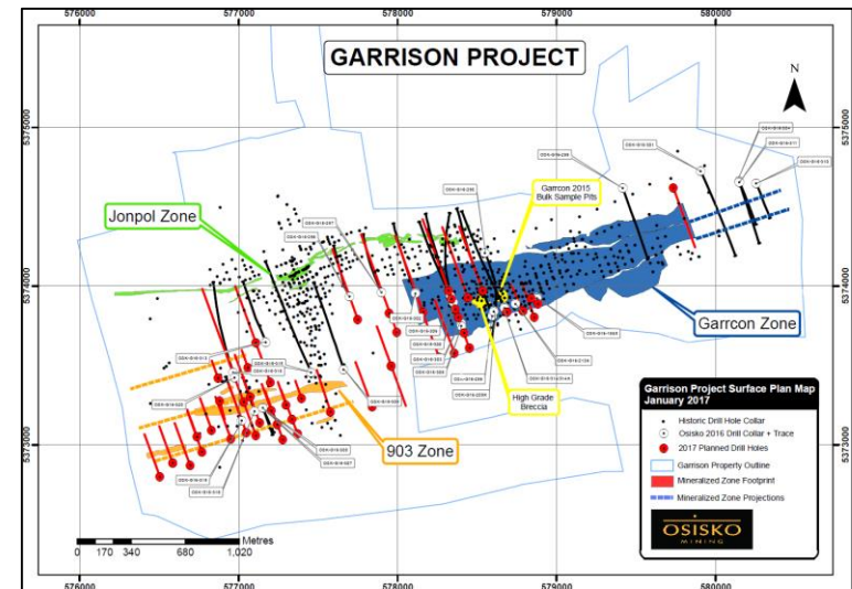
Drilling Program
