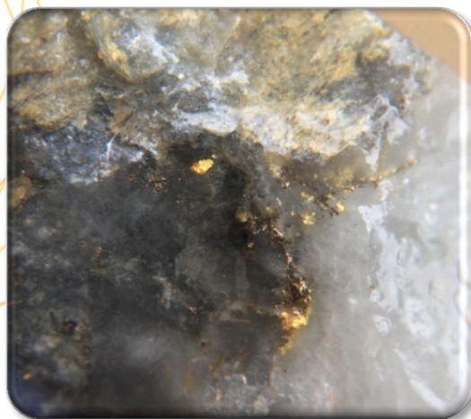
Visible Gold in Diamond Hole XDD006 at 126m depth
